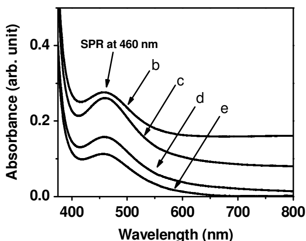
Fig. 11 - Gradual evolution of SPR band of bismuth nanometals in bismuth oxide glasses with increasing oxidizing increasing \text{KNO}_3 concentration used as oxidizing agent in their synthesis instead of conventional reducing agent (adapted from Ref. 71)
