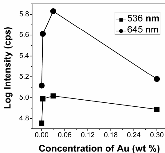
Fig. 18 - Plot of log intensity as a function of concentration of Au (wt %) for 536 and 645 nm emission bands. (adapted from Ref. 119).
